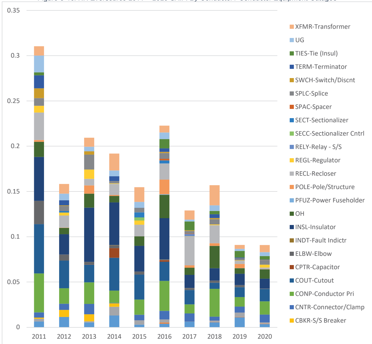
Figure 5-46. NH Eversource 2011 – 2020 SAIFI By Conductor / Conductor Equipment Outages
